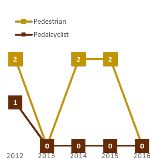
Non-Motorist Fatalities
