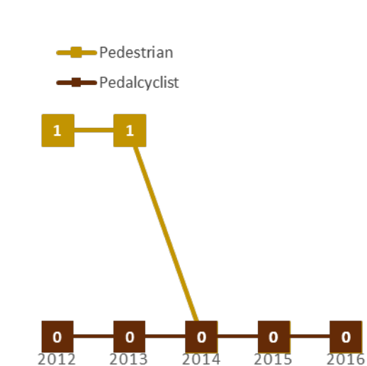
Non-Motorist Fatalities
