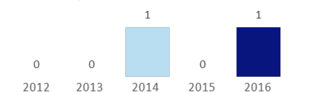
Motorcyclists Fatalities
